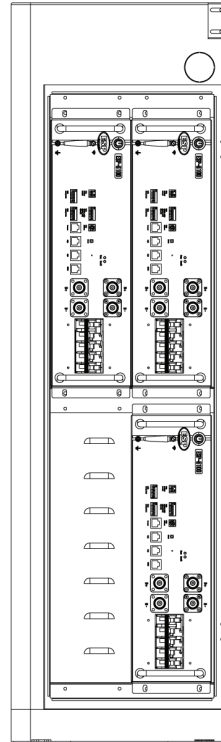
3 Battery Pack Configuration
