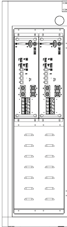
2 Battery Pack Configuration
