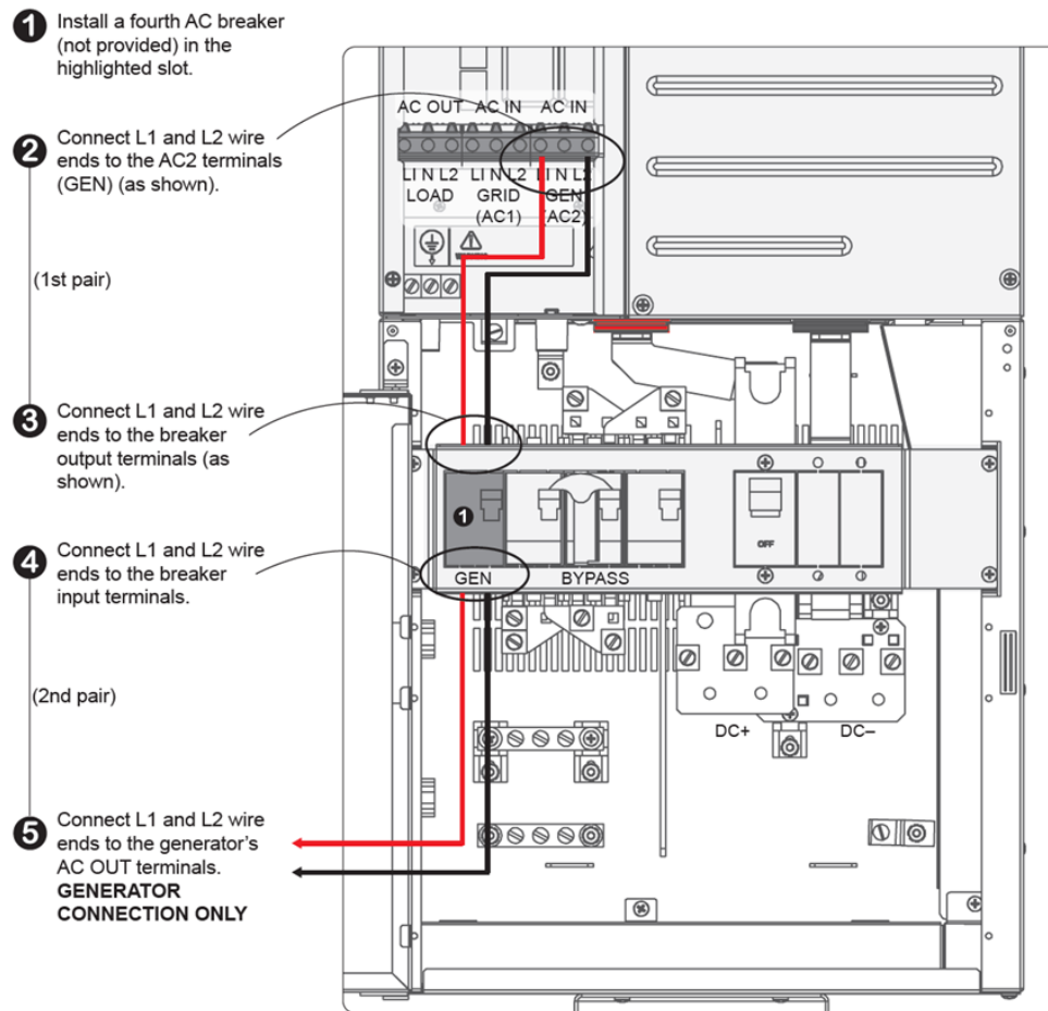
Figure 8.0 – Optional Generator Installation/Connection Diagram
