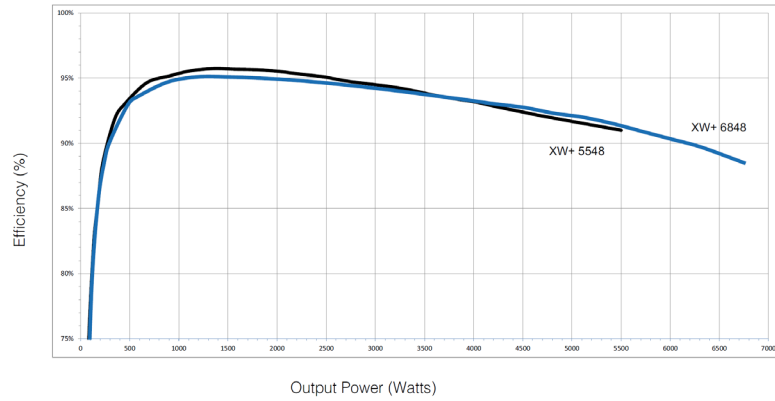
Figure 19.0 - Conext WX+ Efficiency vs Load Graph
