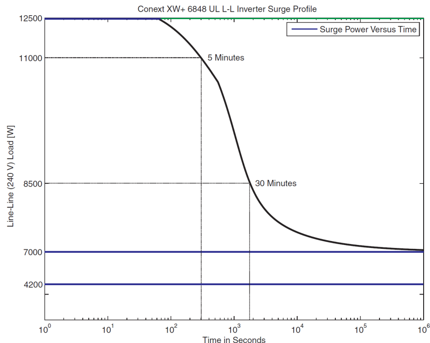
Figure 16.0 – Conext WX+ Operating Time vs 240VAC Load Graph
