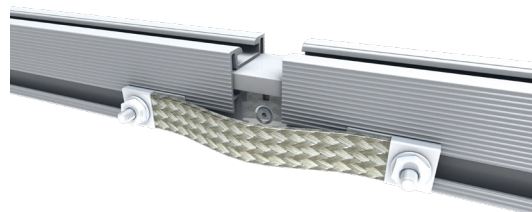
Images 5.2.12 WEEB-BNDJMP8.0 installed with Internal QSplice
