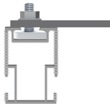
Image 6.1.1 Rail/MLPE Attachment
