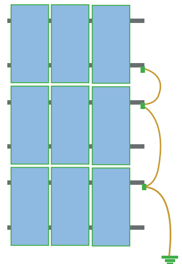
Image 2.5.2 Array bonding connections at each module row
