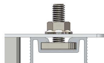
Image 2.4.14 T-bolt in QRail with MLPE installed
