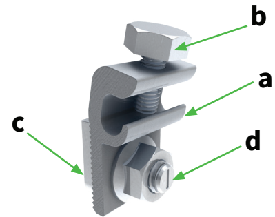
Image 2.5.1 QLug Grounding Lug components T-bolt: 16ft-lbf (22N-m) Wire capture bolt: 6-8 AWG: 60in-lbs (7N-m) 10-12 AWG: 36in-lbs (4N-m)
