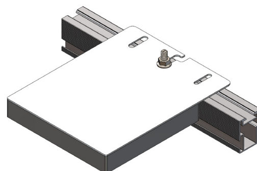
Image 2.4.15 MLPE mounted to QRail with T-bolt.
