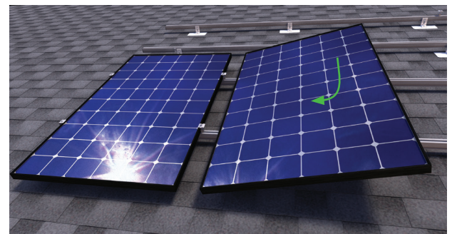
Image 6.4.2 Inner module installation step 2
