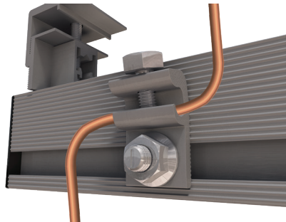
Image 2.5.3 Lug installed in side channel
