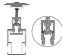
Image 2.4.5 Clamp hooks and rail
