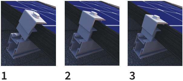
Image 6.3.3 End Clamp installation
