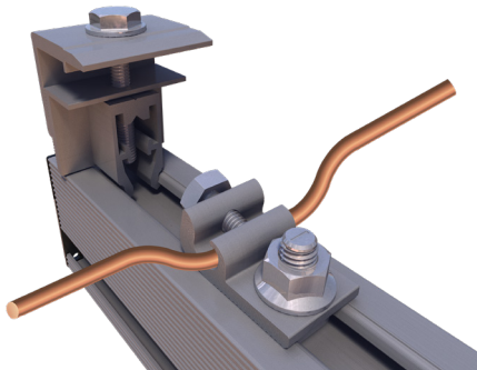
Image 2.5.4 Lug installed in top channel
