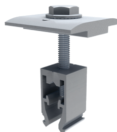
Image 2.4.7 Bonding plate mid clamp [12 ft-lbf (16 N-m)]
