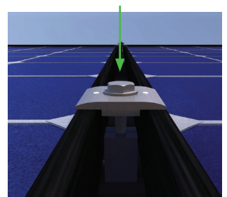
Image 6.4.4 Tighten clamp bolt [12 ft-lbf (16 N-m)]
