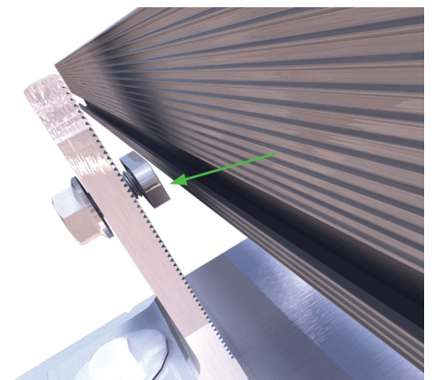
Image 5.3.2 T-bolt correctly positioned for insertion
