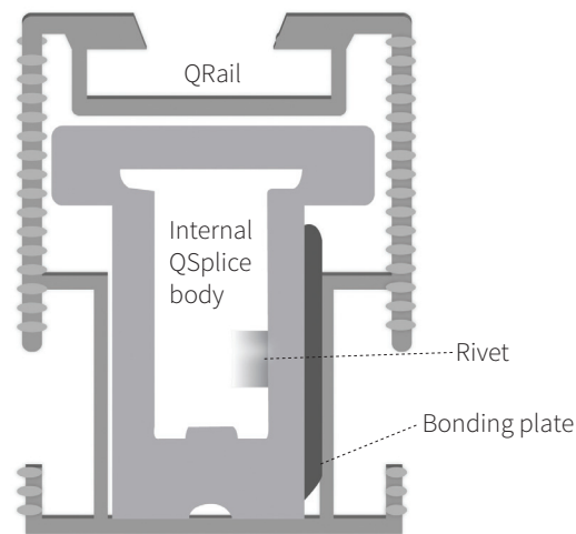
Image 2.4.11 QRail Internal QSplice
