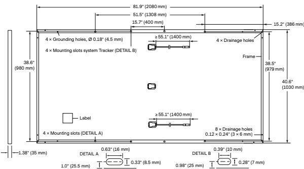
Fig. 1: External dimensions (in inch (mm)) and components for Q.PEAK DUO L-G8 and Q.PEAK DUO L-G8.3
