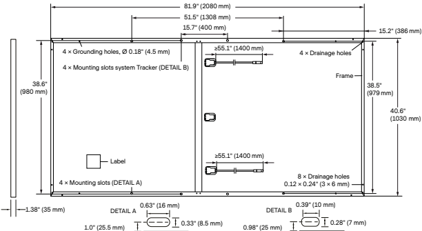
Fig. 2: External dimensions (in inch (mm)) and components for Q.PEAK DUO L-G8.1 and Q.PEAK DUO L-G8.2
