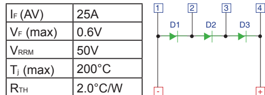
Diode specification and configuration
