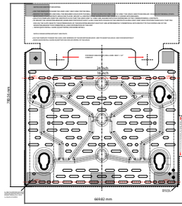
1 × Drill template
